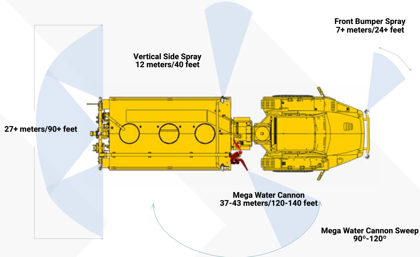
Spray Head Configuration Flow Rates-Mega M3 Water Pump
